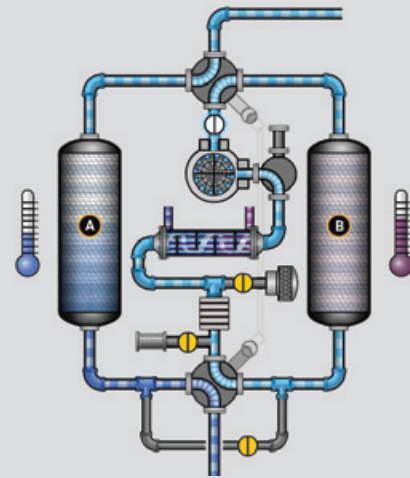
WVM dryer with steam heat exchanger and additional electrical heating element.
