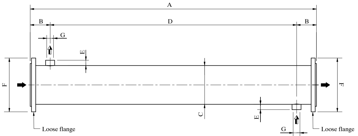
Fig. 2 – Overall dimensions
