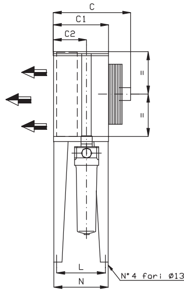
Fig. 4 – Overall dimensions Aftercooler + Separator STH/SFH
