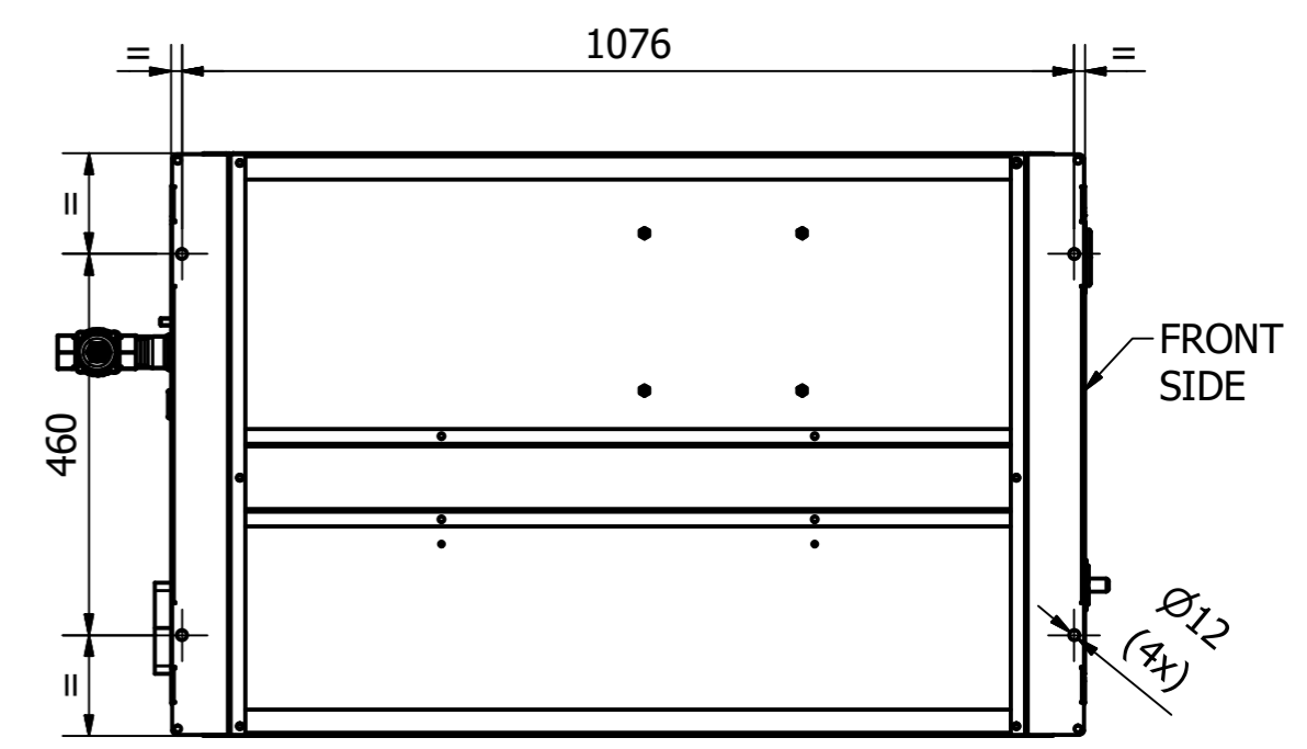
BOTTOM VIEW BASE FIXING HOLES POSITION
